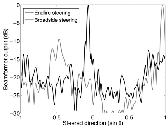
FIG. 6. Array beamformer output as a function of steering angle from array broadside 0^\circ shown for two distinct time instances. Sperm whale clicks with relative bearing 3.7^\circ near array broadside and 73.7^\circ near array endfire. The corresponding 1-dB beamwidths are approximately 1.7^\circ near broadside and 8.0^\circ near endfire. Rectangular window was applied across the array aperture.
